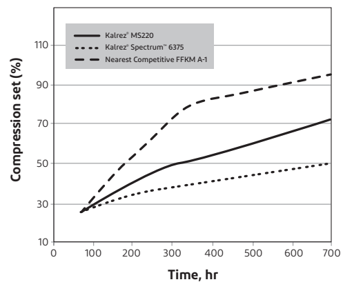
Compression set vs. Time at 204 °C (400 °F)
